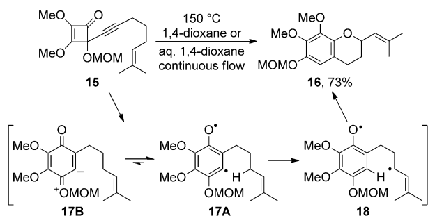
Scheme 3. Influence of OH protection on the reaction course. MOM = methoxymethyl.
