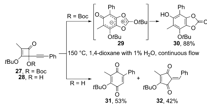
Scheme 6. A new route to catechol carbonates and the influence of alcohol protection on the course of the reaction. Boc = tert -butoxycarbonyl.
