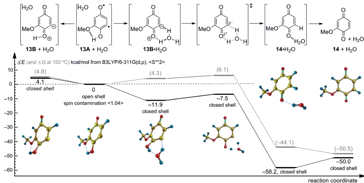
Figure 1. A computational study reveals an orbital isomer switch triggered by water.
