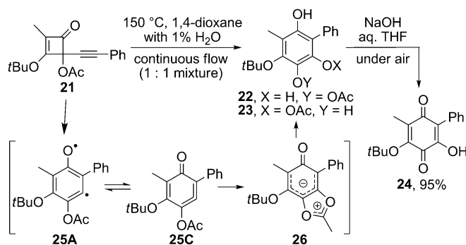
Scheme 5. Experimental evidence that the closed-shell orbital isomer of 25 exhibits cyclohexatrieneone character.
