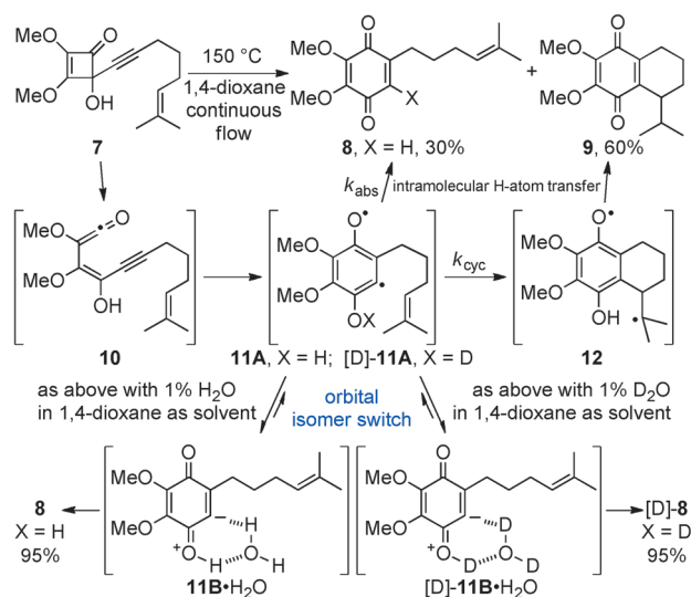
Scheme 2. An orbital isomer switch promoted by water (or D 2 O) diverts the course of the reaction towards the quinone 8 (or [D]- 8 ).
