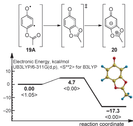
Figure 3. A computational study of the reactivity of the diradical 19A .
