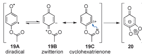
Scheme 4. A computational study predicts the cyclization of the acetate 19 into zwitterion 20 via a closed-shell transition state.
