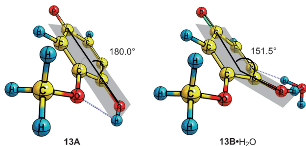
Figure 2. Planarity in diradical 13A contrasts with the pronounced puckering observed for the zwitterion 13B ·H 2 O.
