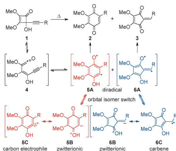
Scheme 1. A prototypical alkynylcyclobutenone rearrangement showing the diradical intermediates and their orbital isomers.
